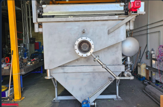
Front view – inlet pipe with recirc line attached, hopper-bottom tank & spherical pressure vessel
