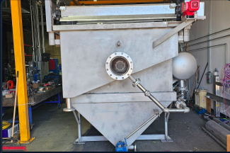
Front view — hopper-bottom tank & spherical pressure vessel
